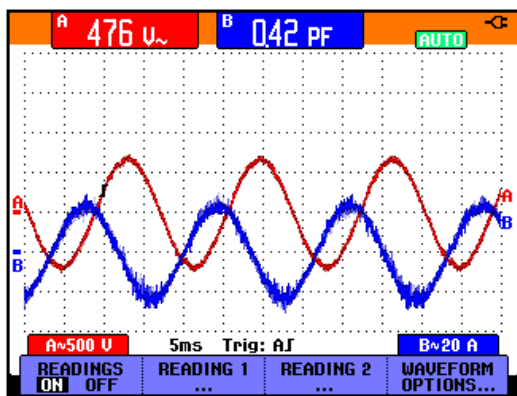
Figure 3b. Compare the waveform alignment and power factor reading between these two examples.
