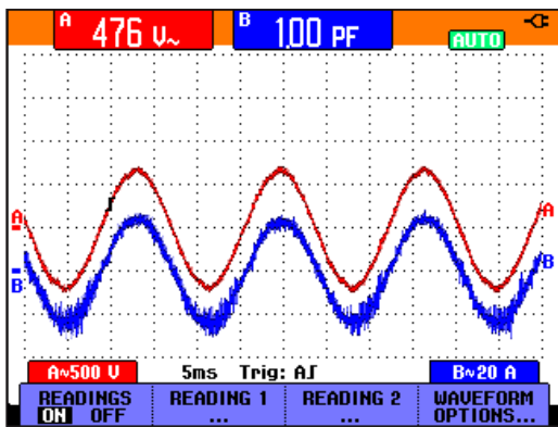
Figure 1. Distortion and line notching are real problems, but are imperceptible with just a meter reading. In this instance, the blue current line is heavily notched.
