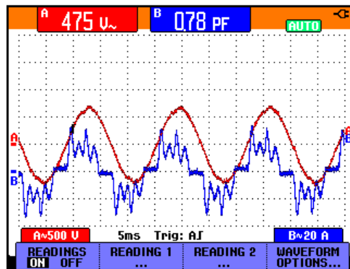
Figure 2. Nonlinear load example.
