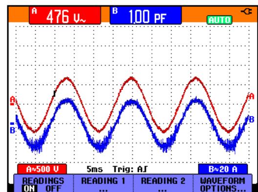
Figure 3a. Good power factor example.
