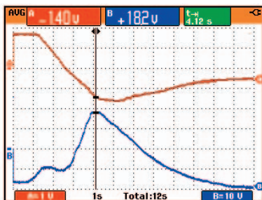
Figure 3 - The position of the feed-scroll (trace A red) and behavior of the hydraulic pressure (trace B blue) shown as a function of time (Fluke 199C).
