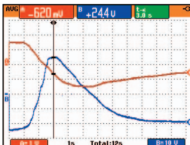
Figure 4 - The position of the feed-scroll (trace A red) and course of the cavity pressure in the mold (trace B blue) shown as a function of time (Fluke 199C).
