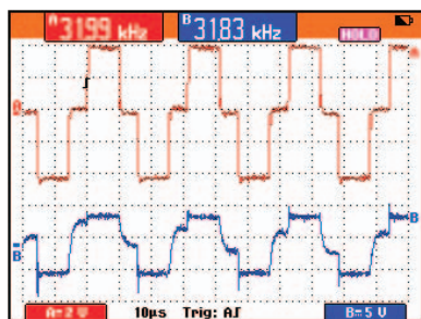
Figure 3. A ScopeMeter shot of SkyLine's CO timing source provides graphic detail that reveals an improper signal termination. The source signal in trace A shows the crisp edges and "shoulders" of a good signal. Trace B has the same frequency as trace A, and is in phase with trace A, but its edges and shoulders are not nearly as "clean". These indicators suggest improper signal termination.
