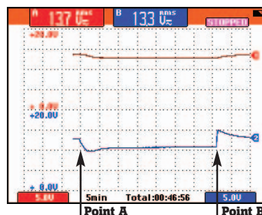
Figure 2. A check of cells from two independent batteries reveals a fault with Battery 2 (trace 2). A charger is removed from both batteries at Point A. Battery 1 holds its charge, but Battery 2 shows a precipitous drop in voltage. At Point B, the charger is placed on both batteries again, but the fault with Battery 2 remains evident.
