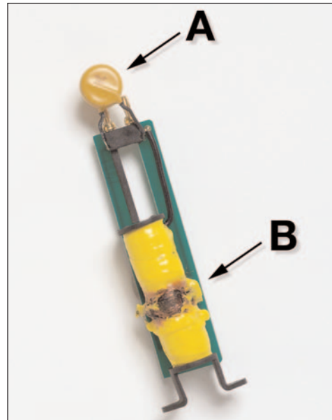
Figure 1: This solenoid tester experienced a catastrophe failure after receiving an impulse. Even with an MOV (metal oxide varistor) (see A), the unit will still self-destruct from overheating (see B).
