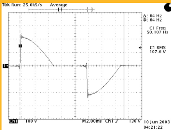
Phase-fired waveform
